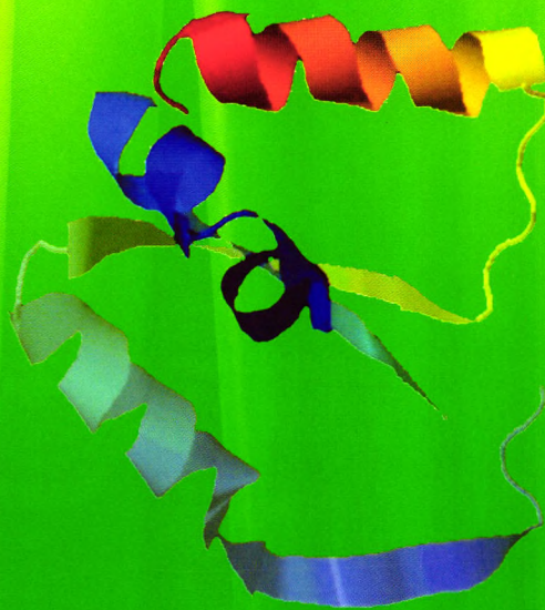
Predicted three-dimensional structure of DR_2566 protein (P.020201)
