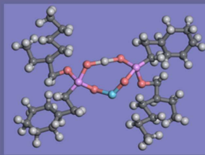
Interaction with La 3+ ion
