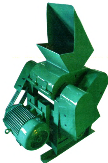
9P-20型饲草秸秆块破丝机
